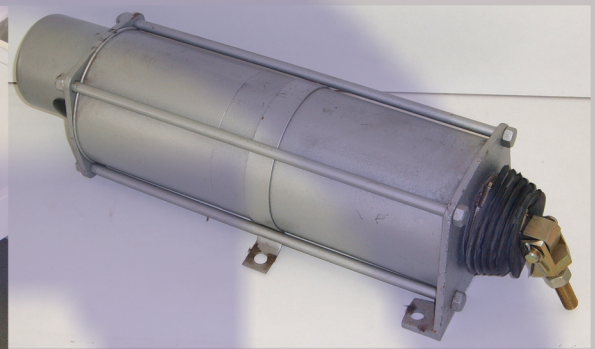
PNEUMATIC CYLINDER FOR PANTOGRAPH LANDING
