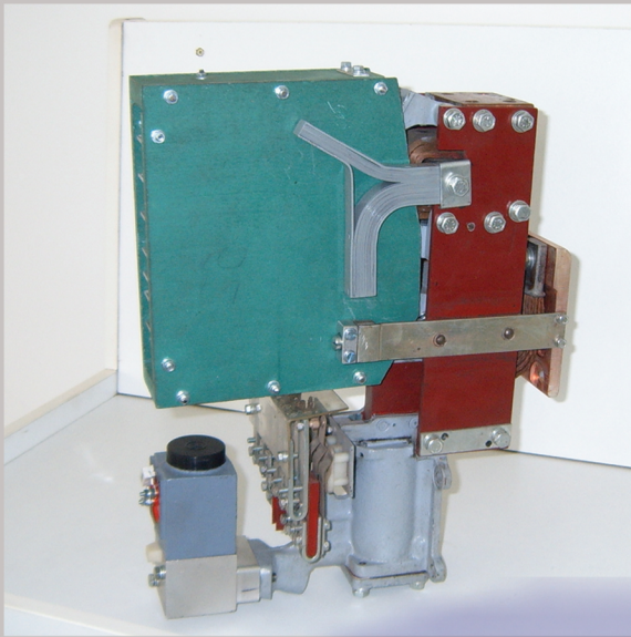
CONTACTOR KN-5213 electro-pneumatic single-pole contactor
