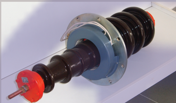
ROOF BUSHING INSULATOR KPI-30 roof bushing insulator with current transformer
