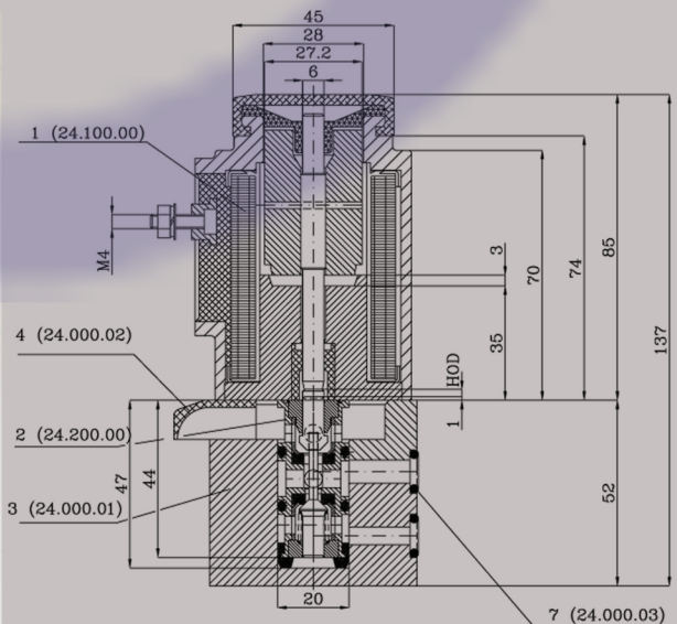
MAGNET VALVE EP-10, EP-20, EP-30
