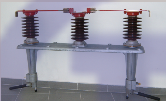
PANTOGRAPH DISCONNECTER RSP 25 installed on the roof of electric locomotive
