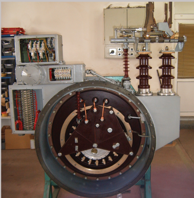
TAP CHANGER RTN-25 discontinual regulation in 41 degrees on the high voltage transformer side
