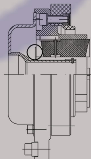
EARTHING DEVICE UKS-1
