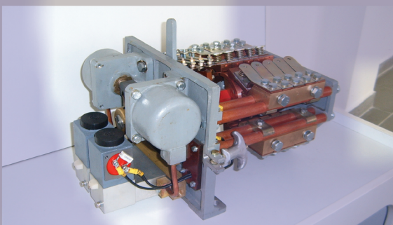
REVERSING SWITCH DKJK-V/A
